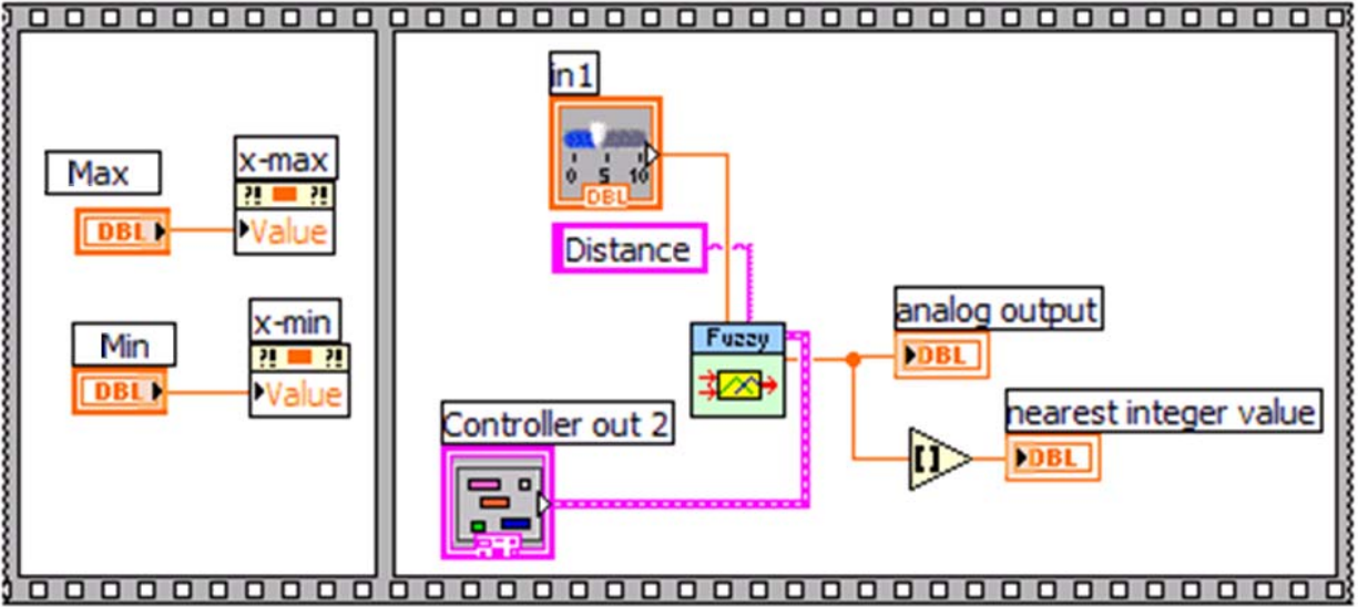
Figure 7. Block code to obtain the steering angle code from the 'max' and 'min' values
