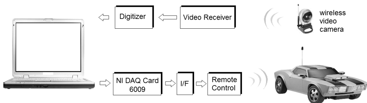
Figure 1. Block diagram of the autonomous vehicle navigation system.
