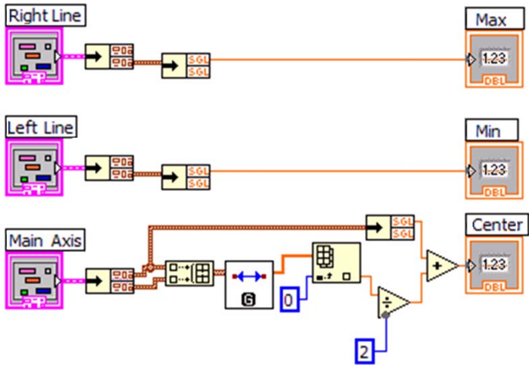
Figure 6. Sub-virtual instrument ‘fuzzy’
