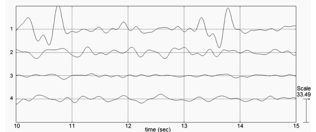
Fig. 11. Separated signals obtained from the ICA algorithm.
