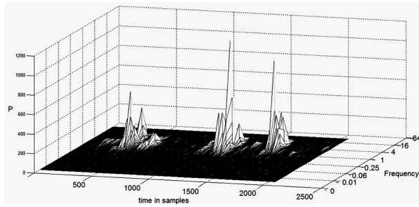
Fig. 12. Scalogram of signal from channel 2.
